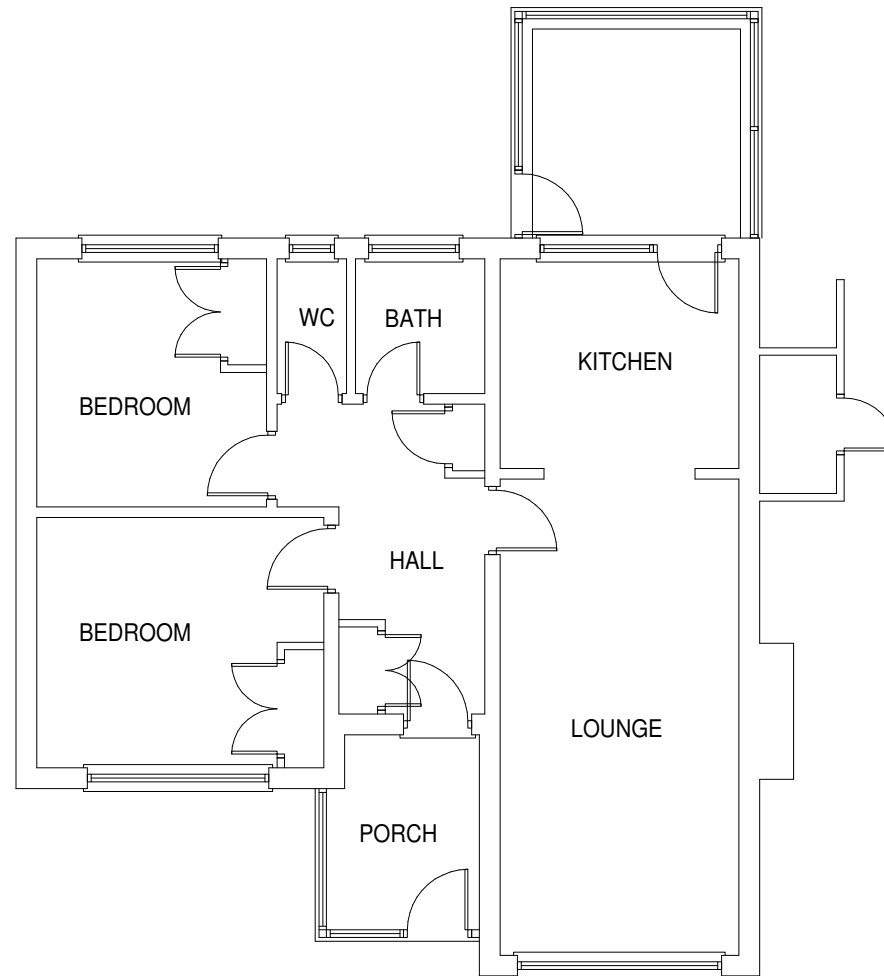
Existing Ground Floor Plan (scale 1:100@A3)
